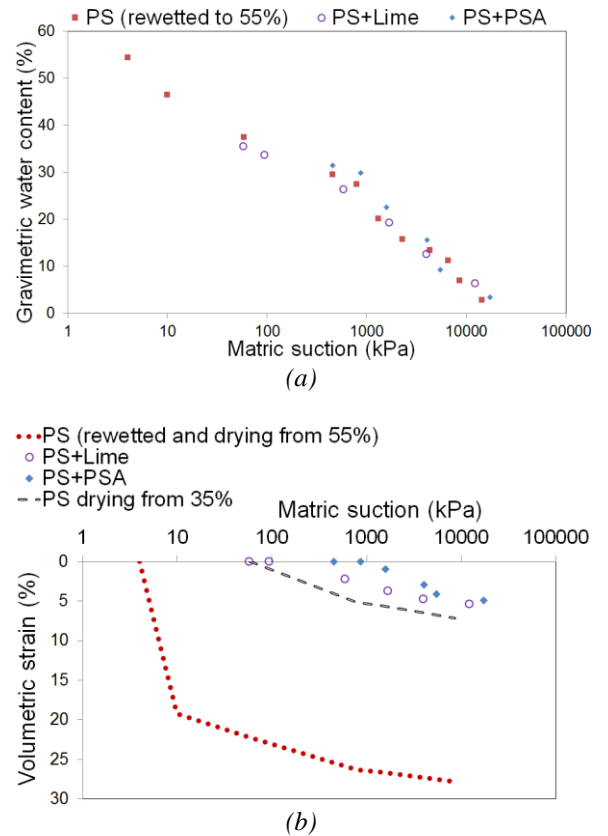
Figure 4 (a)-(b). Filter paper testing results (drying curves): (a) water content vs. matric suction; (b) volumetric strain upon drying vs. matric suction
