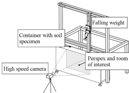
Figure 1. Schematically setup of the laboratory investigation.
