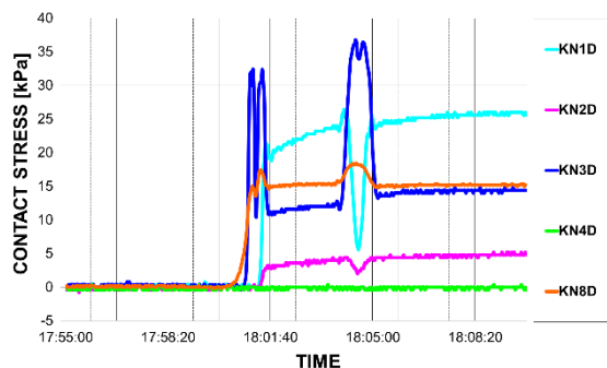
Figure 4. The contact stress during the field test.
